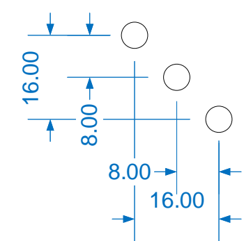
Diagonal hole details.
